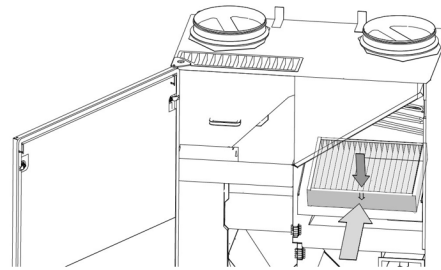
Innerfilter (intagsfilter)
