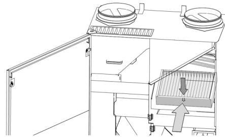
Innerfilter (intagsfilter)
