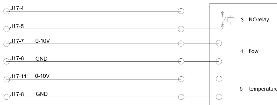
Figur 17: Analog BMS
