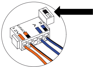
Figur 25: DIP-omkopplare sluten (ON)
