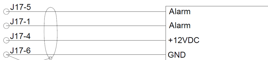
Figur 12: PIR sensor
