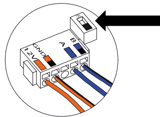
Figur 26: DIP-omkopplare öppen (OFF)
